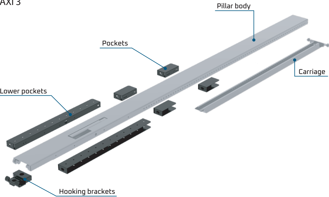
Pillar MAXI 3 fix position
